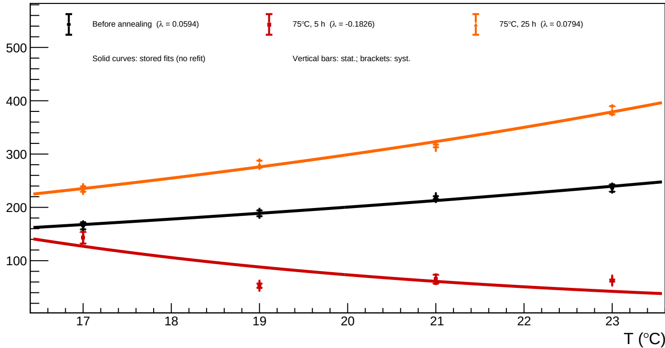
A1_v=5 - Spot 35 (x = 1227.63, y = 666.40): luminosity vs temperature for all annealing phases
