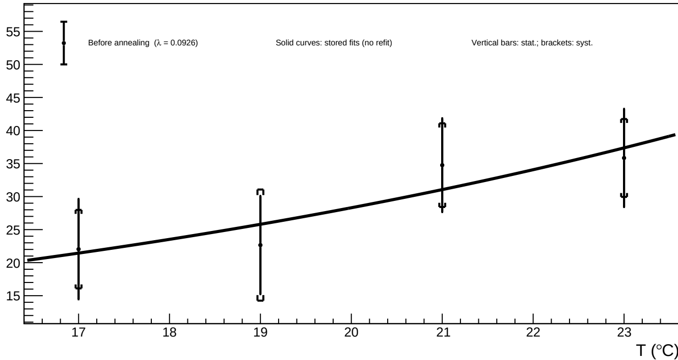
A1_v=5 - Spot 39 (x = 1255.56, y = 231.78): luminosity vs temperature for all annealing phases
