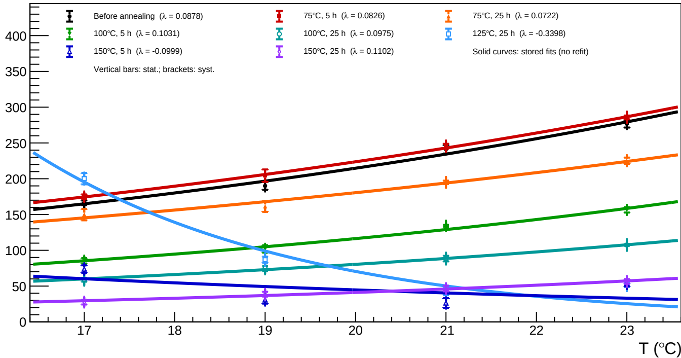
A1_v=5 - Spot 45 (x = 1372.33, y = 810.33): luminosity vs temperature for all annealing phases
