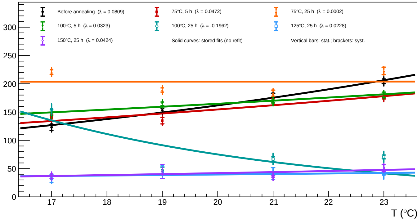
A1_v=5 - Spot 46 (x = 1375.59, y = 912.08): luminosity vs temperature for all annealing phases
