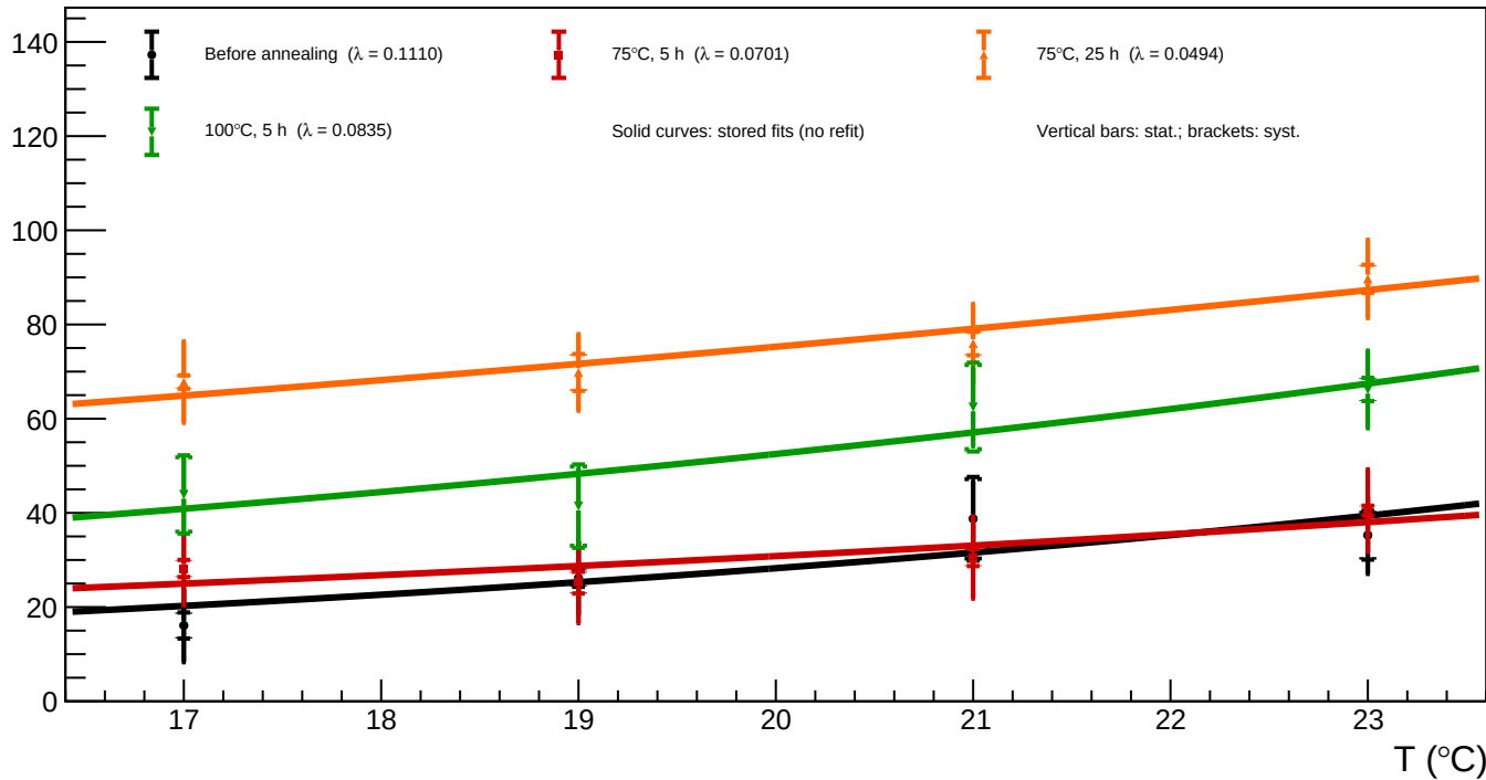
A1_v=5 - Spot 47 (x = 1464.40, y = 944.57): luminosity vs temperature for all annealing phases
