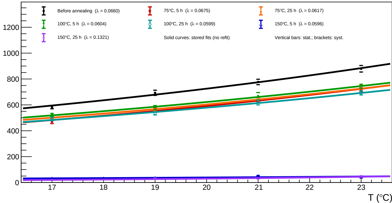
A1_v=5 - Spot 48 (x = 1496.93, y = 507.50): luminosity vs temperature for all annealing phases
