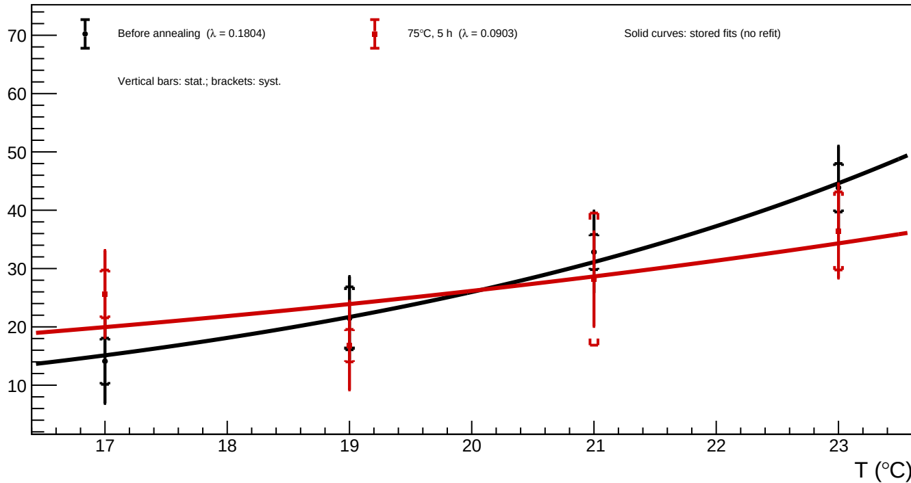
A1_v=5 - Spot 51 ( x = 1584.50 , y = 809.99 ): luminosity vs temperature for all annealing phases
