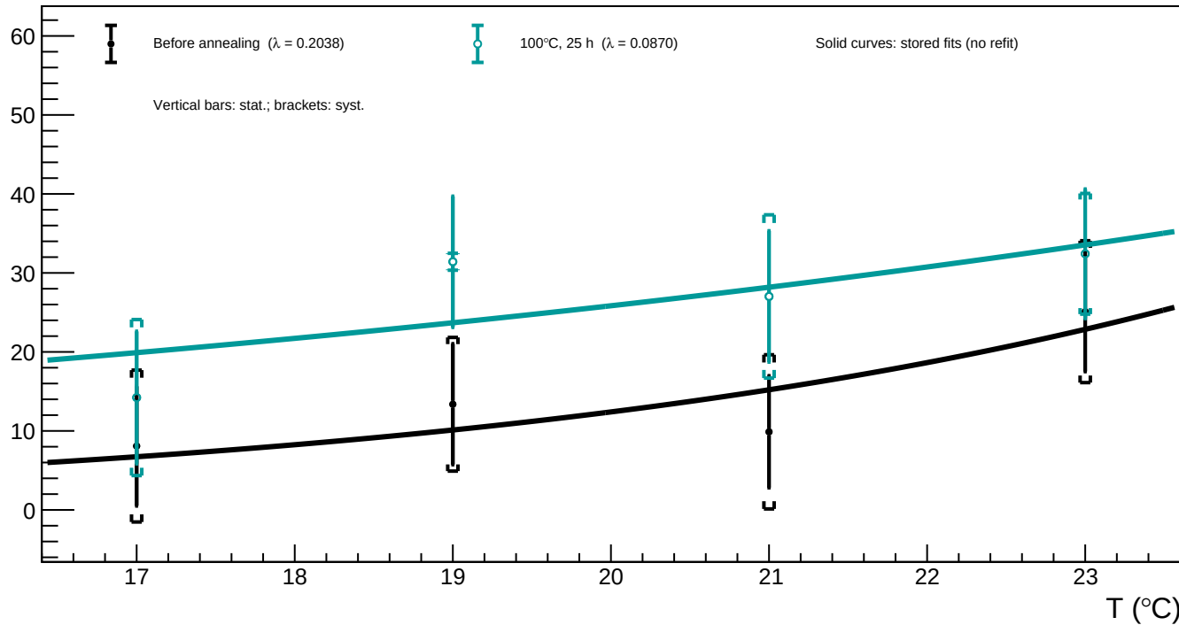
A1_v=5 - Spot 52 (x = 1596.81, y = 321.02): luminosity vs temperature for all annealing phases
