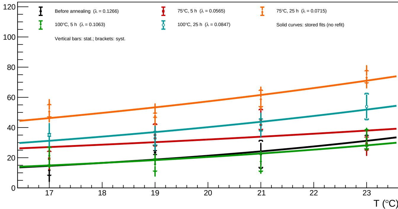
A1_v=5 - Spot 53 (x = 1653.25, y = 629.27): luminosity vs temperature for all annealing phases
