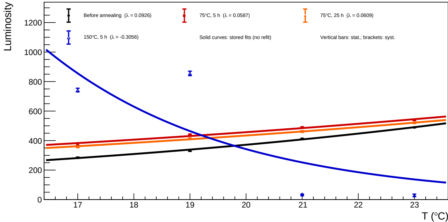
A1_v=5 - Spot 55 (x = 1772.62, y = 478.35): luminosity vs temperature for all annealing phases
