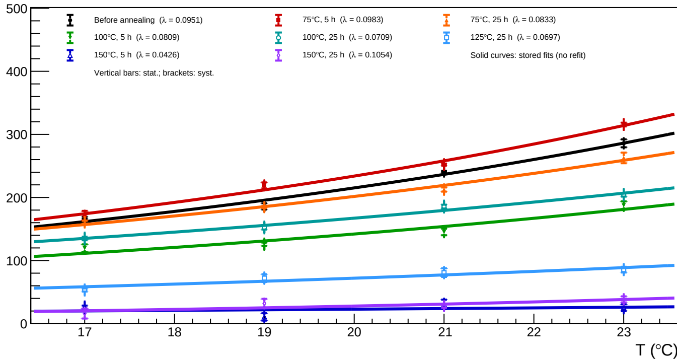
A1_v=5 - Spot 56 ( x = 1782.63 , y = 555.71 ): luminosity vs temperature for all annealing phases
