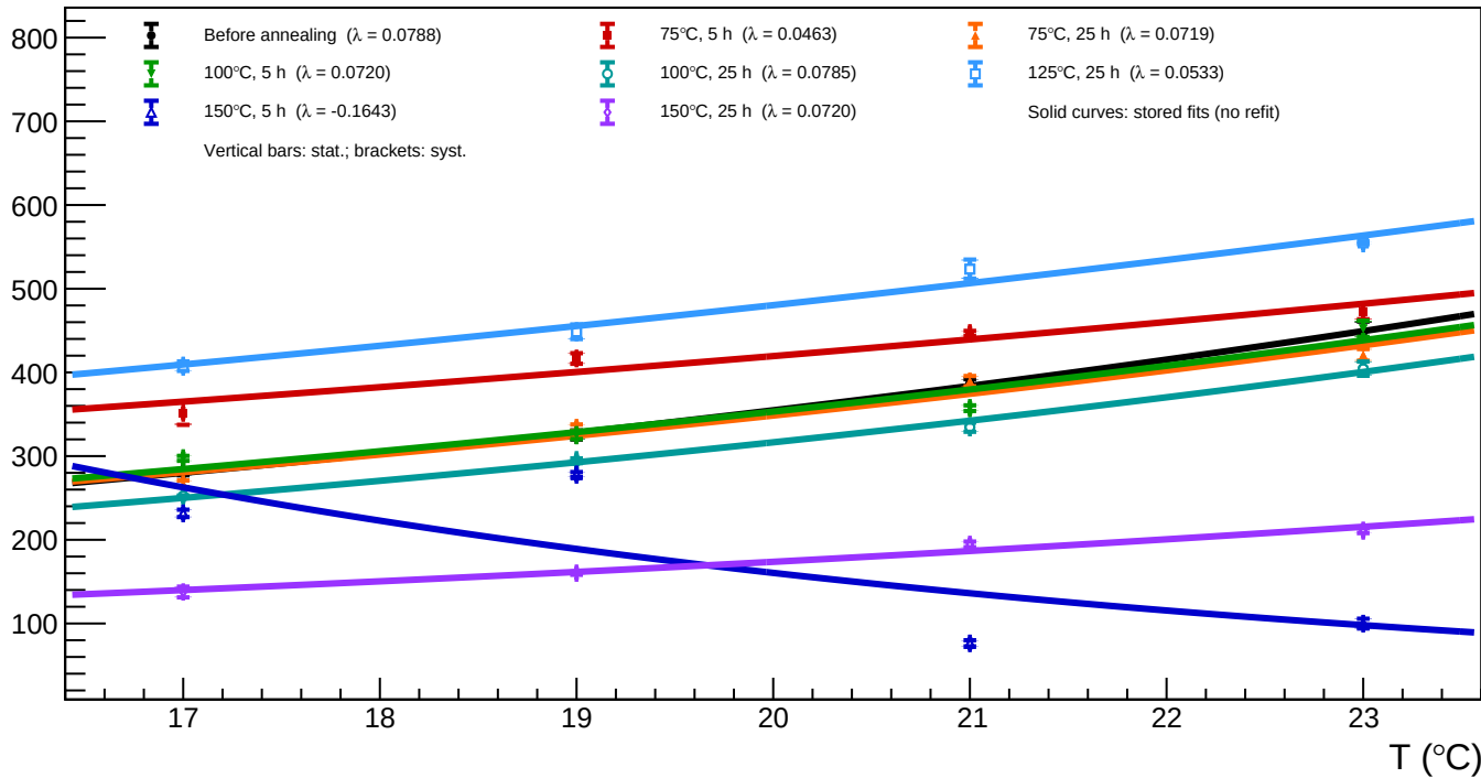
A1_v=5 - Spot 57 ( x = 1821.18 , y = 356.85 ): luminosity vs temperature for all annealing phases
