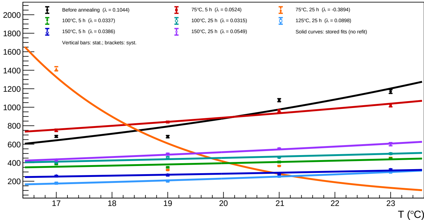
A1_v=5 - Spot 6 ( x = 237.37 , y = 242.33 ): luminosity vs temperature for all annealing phases
