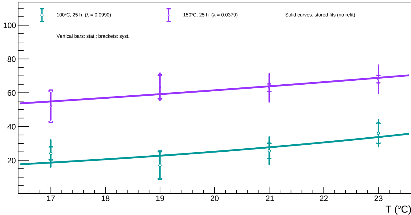
A1_v=5 - Spot 61 (x = 455.82, y = 764.39): luminosity vs temperature for all annealing phases
