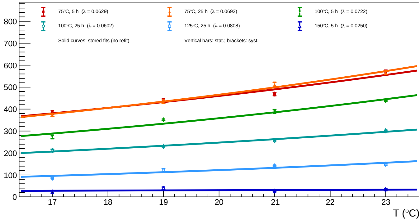
A1_v=5 - Spot 64 (x = 908.33, y = 731.66): luminosity vs temperature for all annealing phases
