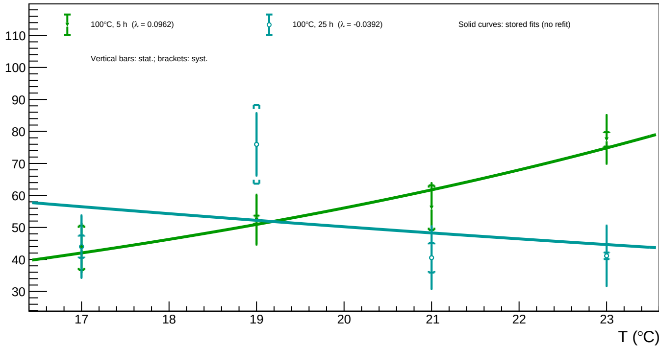
A1_v=5 - Spot 71 ( x = 1387.89 , y = 117.09 ): luminosity vs temperature for all annealing phases
