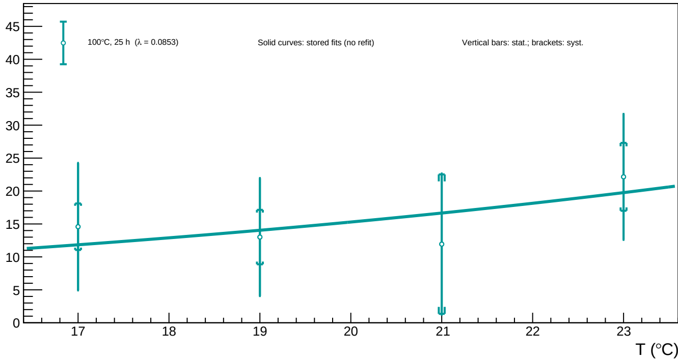
A1_v=5 - Spot 74 (x = 503.50, y = 995.94): luminosity vs temperature for all annealing phases
