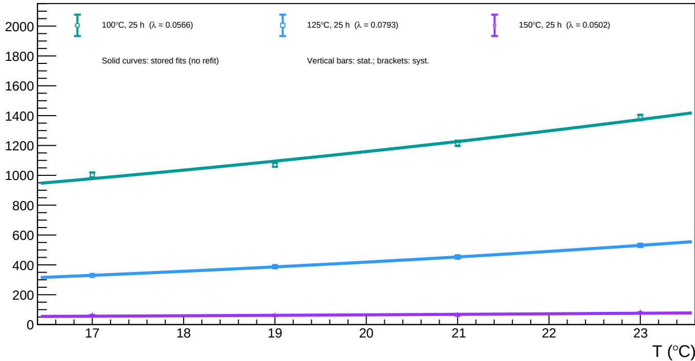
A1_v=5 - Spot 77 (x = 1088.51, y = 519.85): luminosity vs temperature for all annealing phases
