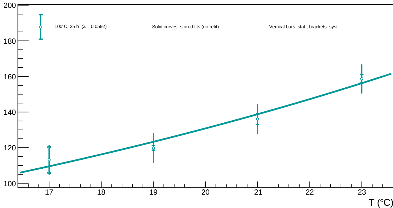
A1_v=5 - Spot 78 (x = 1176.23, y = 649.58): luminosity vs temperature for all annealing phases
