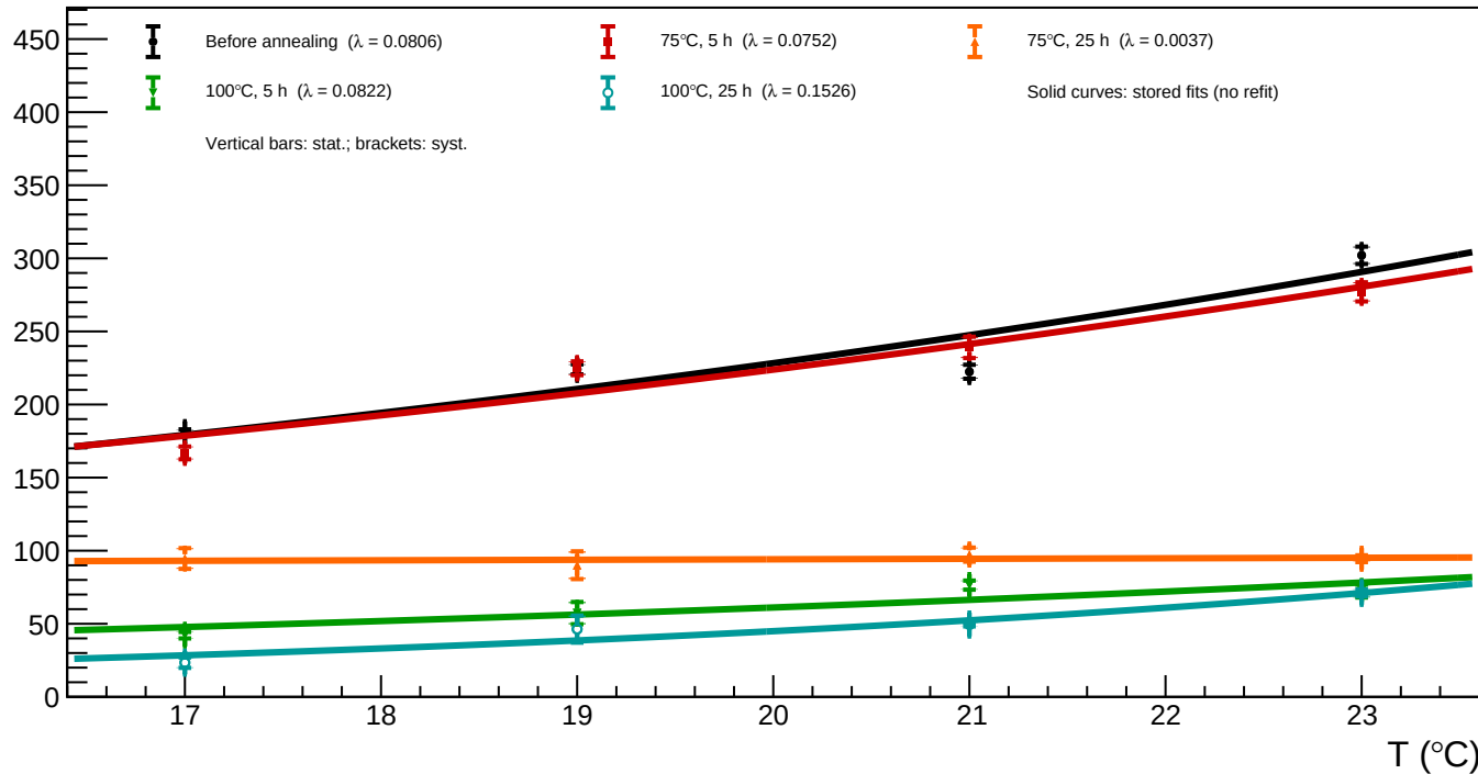
A1_v=5 - Spot 8 (x = 356.51, y = 845.31): luminosity vs temperature for all annealing phases
