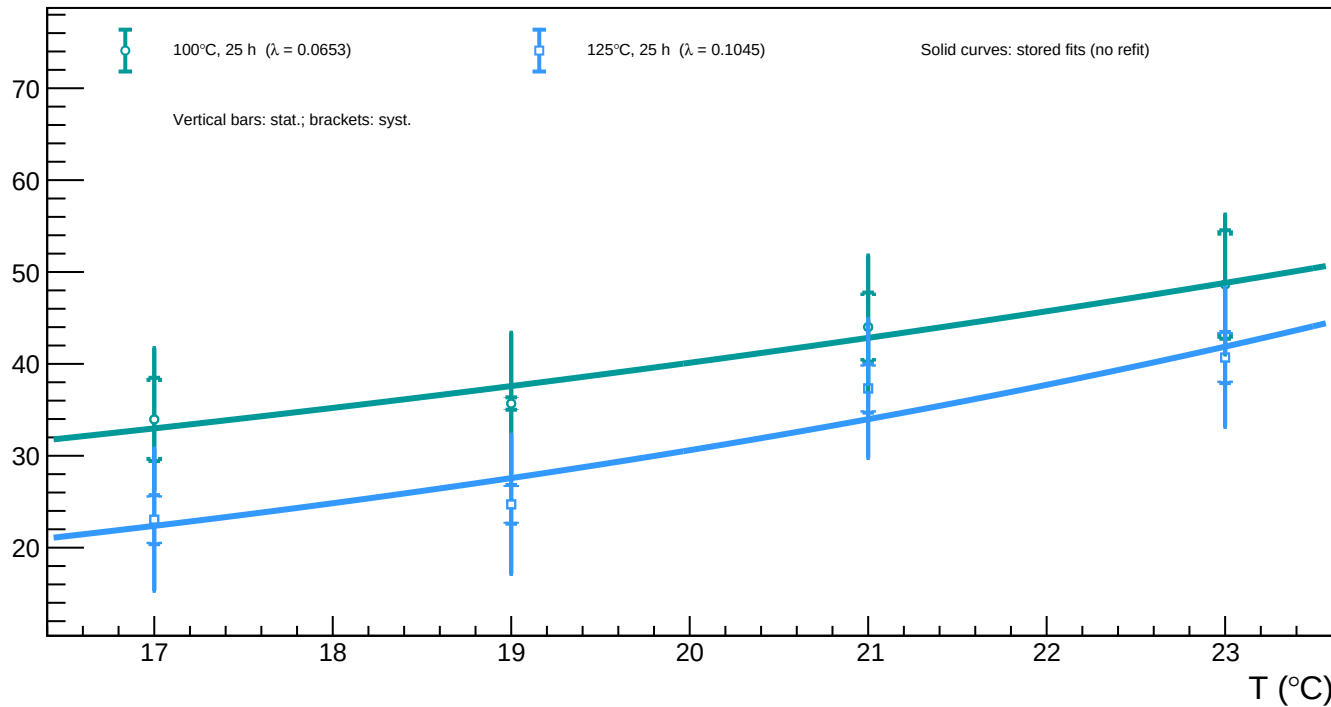
A1_v=5 - Spot 81 (x = 1722.23, y = 803.24): luminosity vs temperature for all annealing phases
