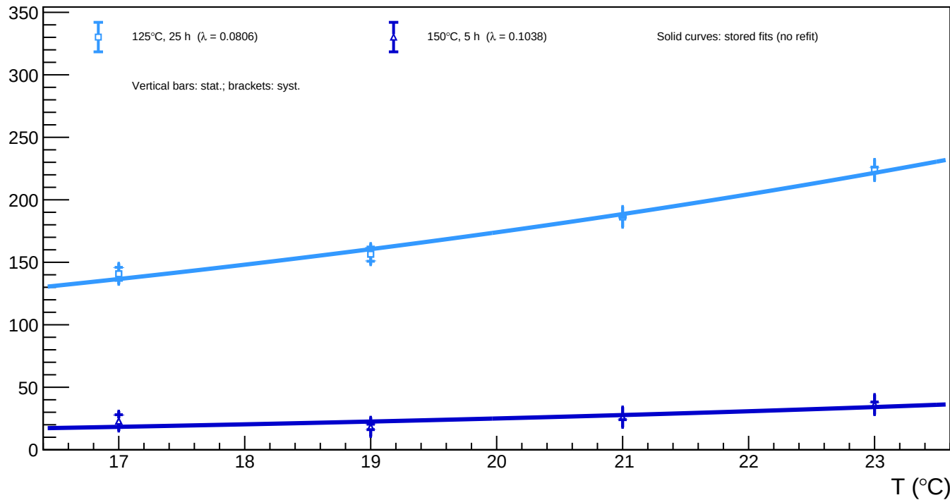
A1_v=5 - Spot 83 (x = 1734.68, y = 908.82): luminosity vs temperature for all annealing phases
