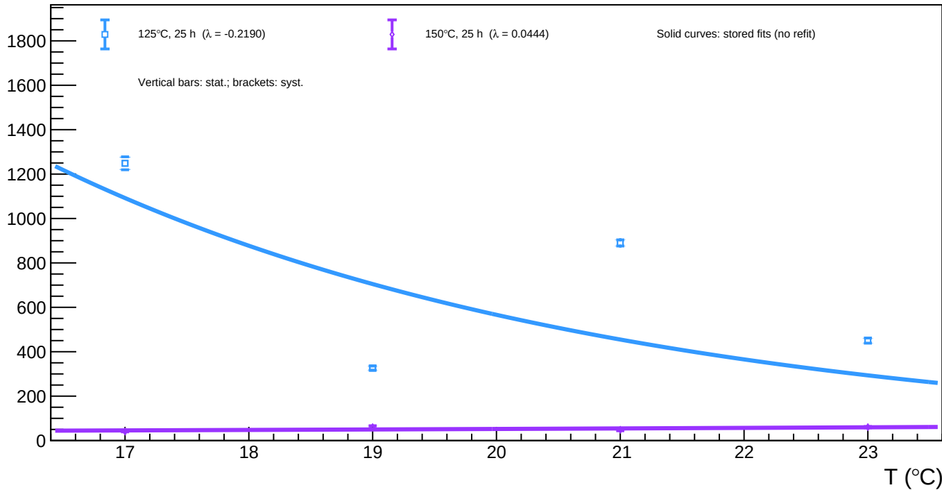
A1_v=5 - Spot 85 (x = 830.57, y = 884.46): luminosity vs temperature for all annealing phases
