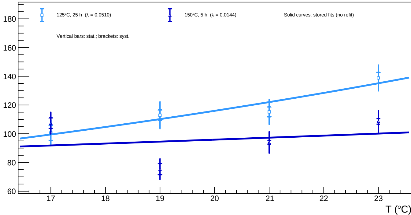
A1_v=5 - Spot 87 ( x = 1557.57 , y = 208.05 ): luminosity vs temperature for all annealing phases
