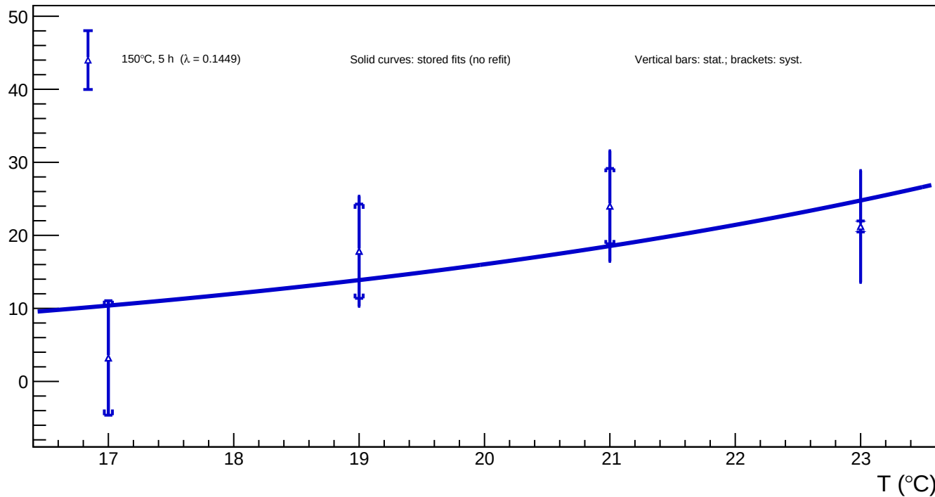
A1_v=5 - Spot 91 (x = 1268.09, y = 787.65): luminosity vs temperature for all annealing phases
