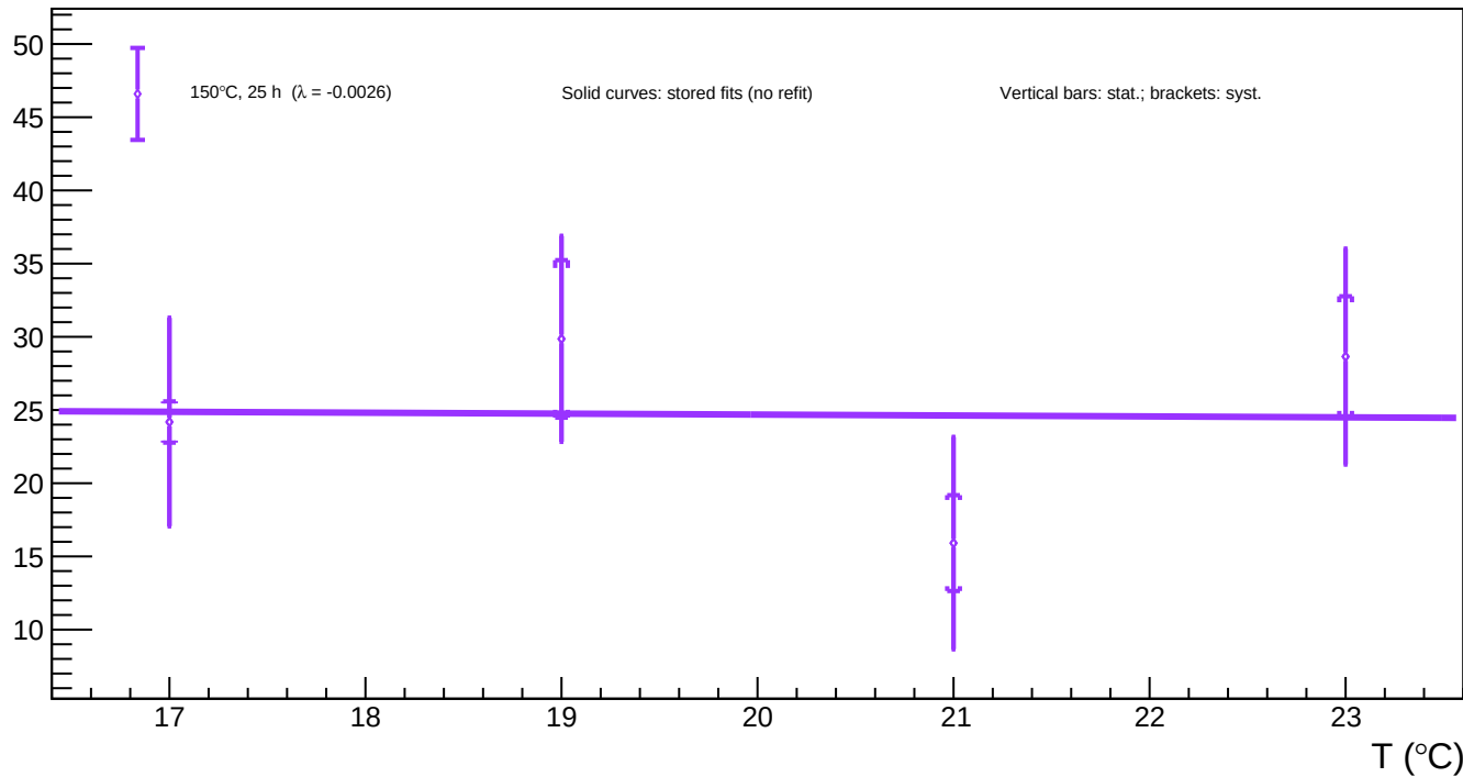
A1_v=5 - Spot 96 (x = 1571.54, y = 682.79): luminosity vs temperature for all annealing phases
