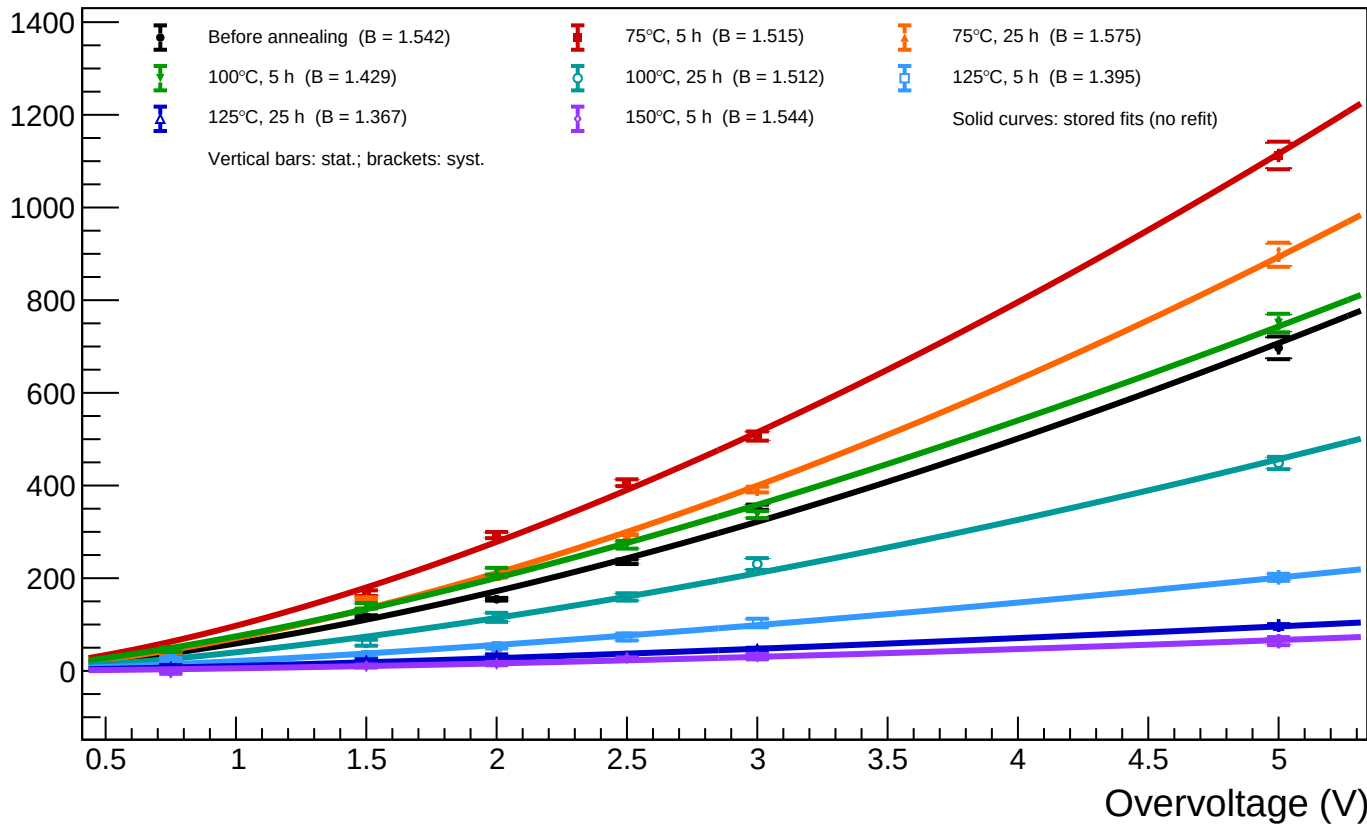
B1_T=20 - Spot 0 (x = 79.86, y = 338.15): luminosity vs overvoltage for all annealing phases
