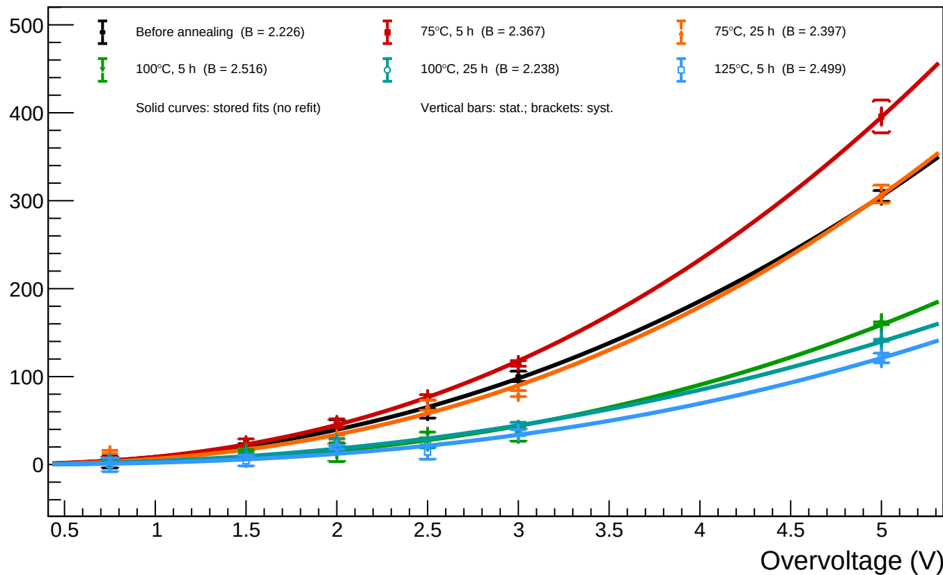
B1_T=20 - Spot 1 (x = 90.95, y = 704.50): luminosity vs overvoltage for all annealing phases
