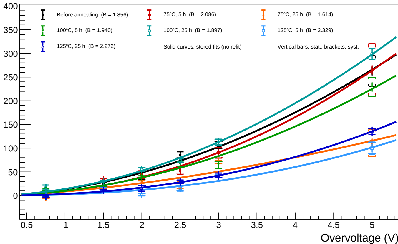
B1_T=20 - Spot 10 ( x = 338.06 , y = 147.53 ): luminosity vs overvoltage for all annealing phases
