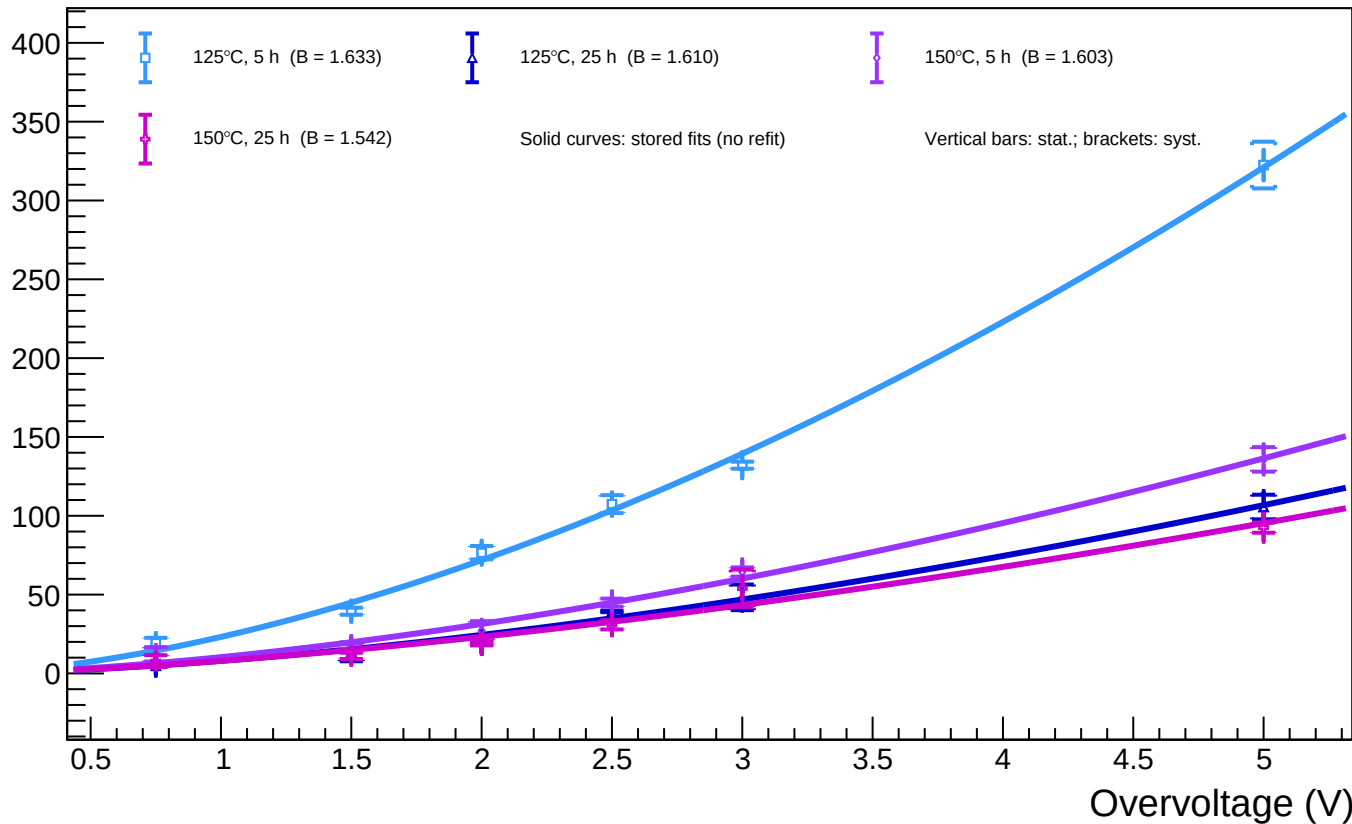
B1_T=20 - Spot 100 (x = 1562.36, y = 887.48): luminosity vs overvoltage for all annealing phases
