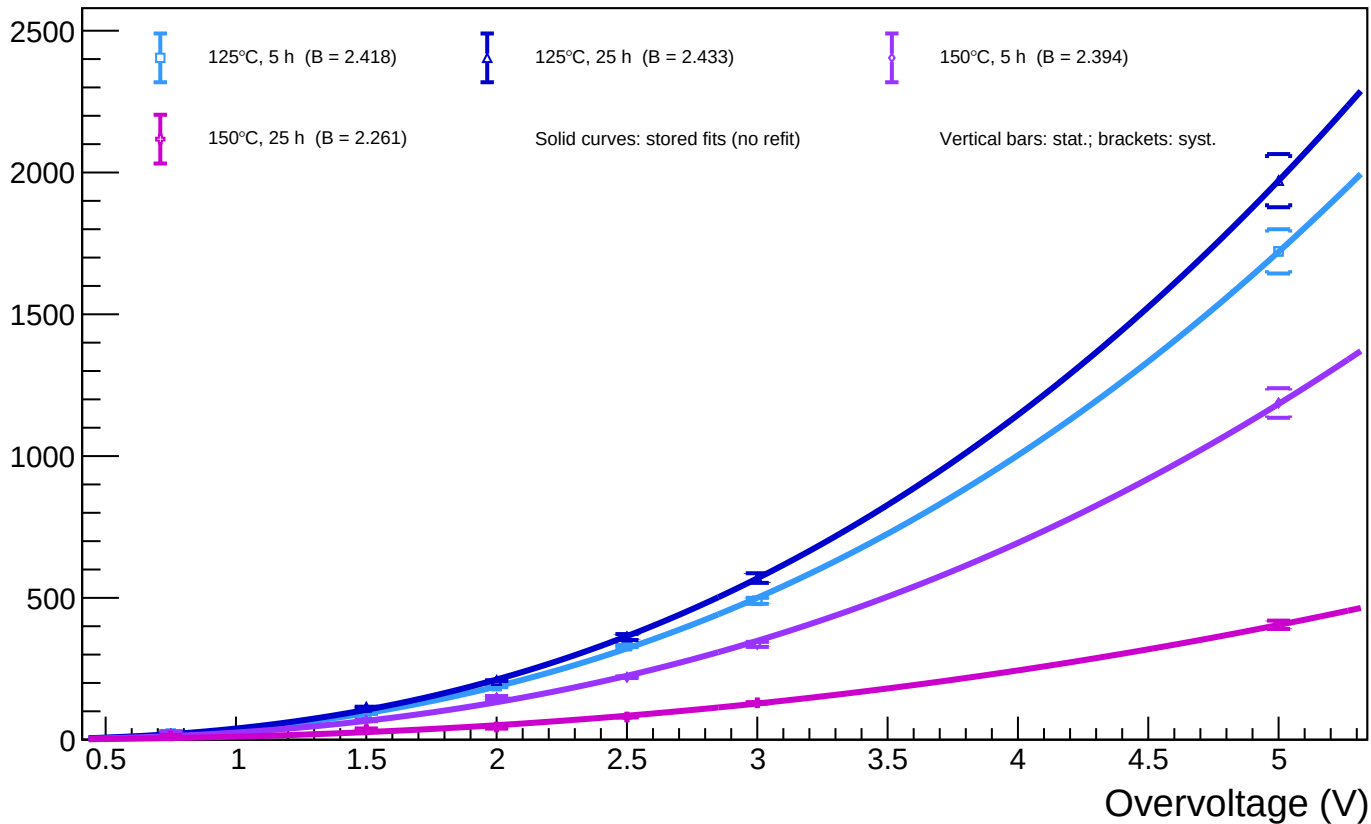
B1_T=20 - Spot 101 (x = 1602.65, y = 812.95): luminosity vs overvoltage for all annealing phases
