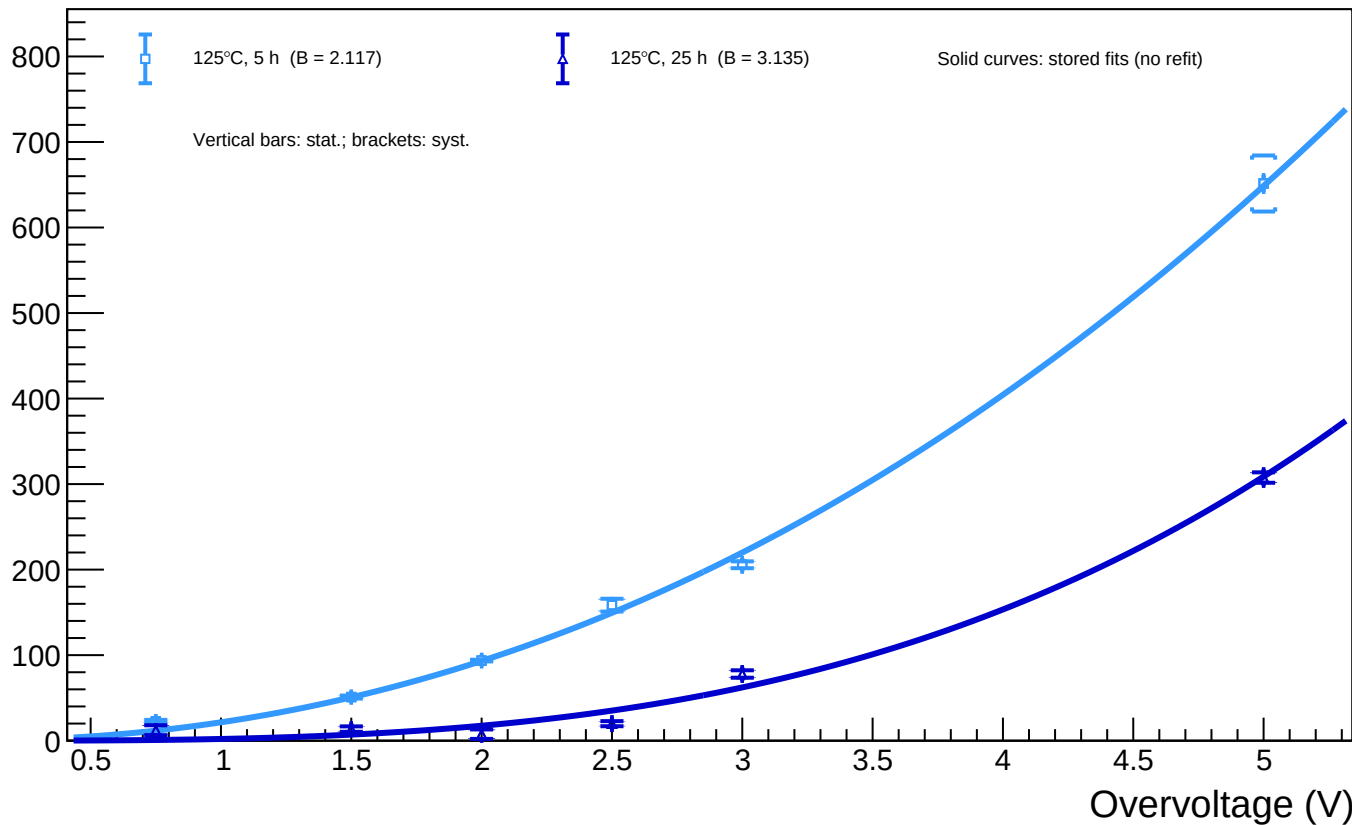
B1_T=20 - Spot 102 (x = 1822.99, y = 904.01): luminosity vs overvoltage for all annealing phases
