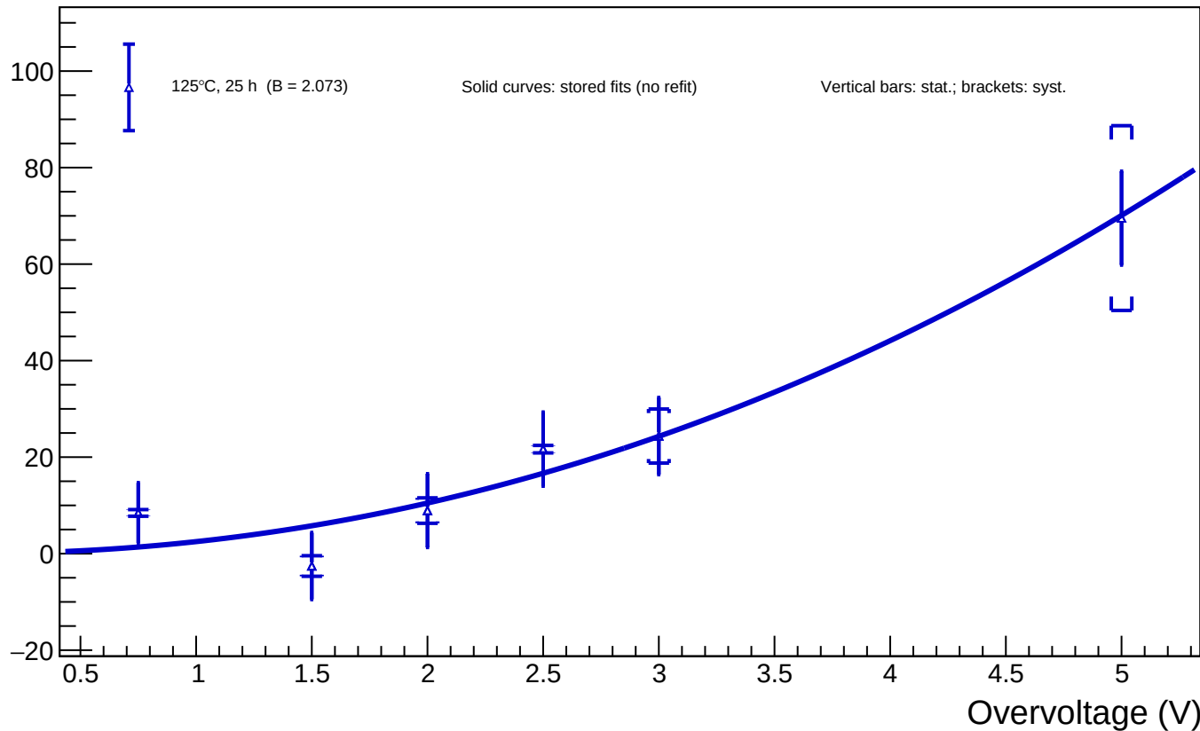
B1_T=20 - Spot 103 (x = 412.11, y = 210.67): luminosity vs overvoltage for all annealing phases
