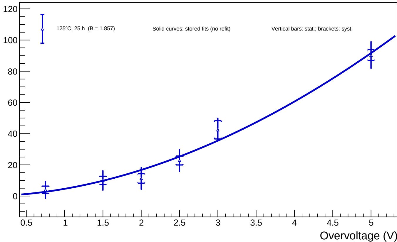
B1_T=20 - Spot 104 (x = 556.93, y = 914.98): luminosity vs overvoltage for all annealing phases
