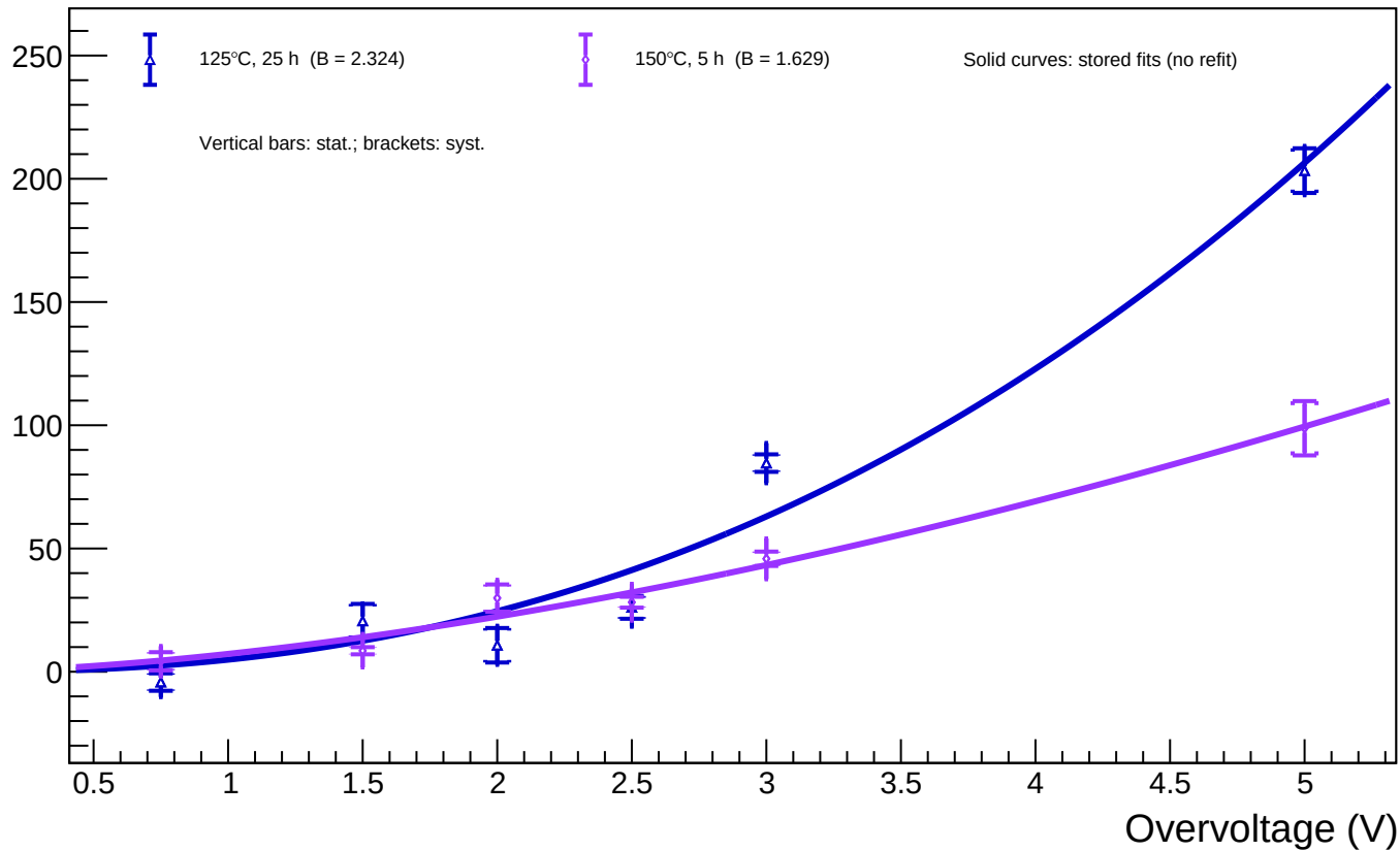
B1_T=20 - Spot 105 ( x = 1237.28 , y = 901.77 ): luminosity vs overvoltage for all annealing phases
