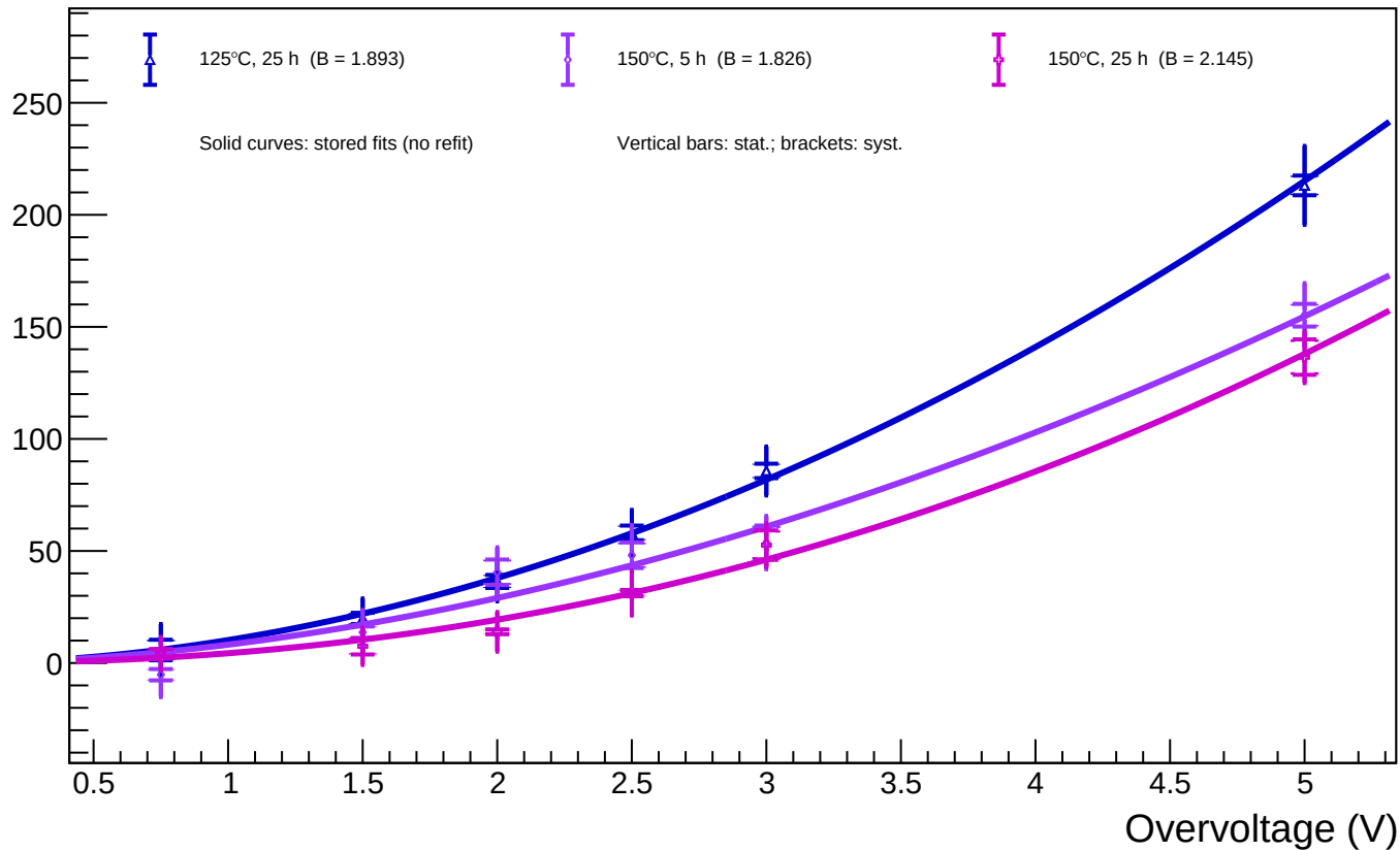
B1_T=20 - Spot 106 ( x = 1345.67 , y = 546.21 ): luminosity vs overvoltage for all annealing phases
