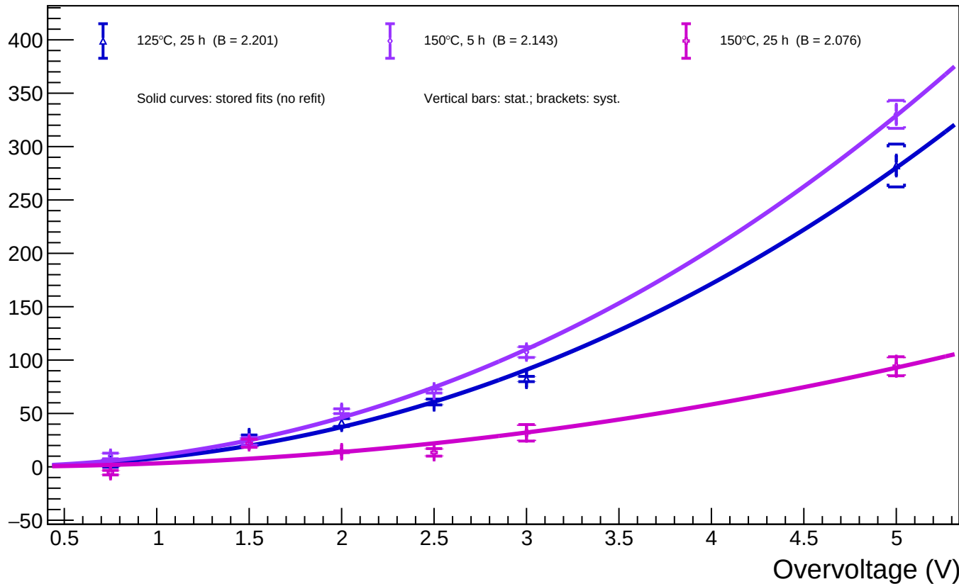
B1_T=20 - Spot 107 (x = 1626.26, y = 630.86): luminosity vs overvoltage for all annealing phases
