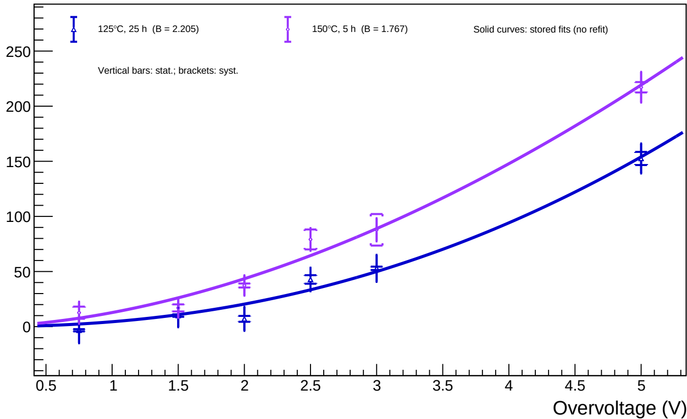
B1_T=20 - Spot 108 ( x = 1689.50 , y = 695.97 ): luminosity vs overvoltage for all annealing phases
