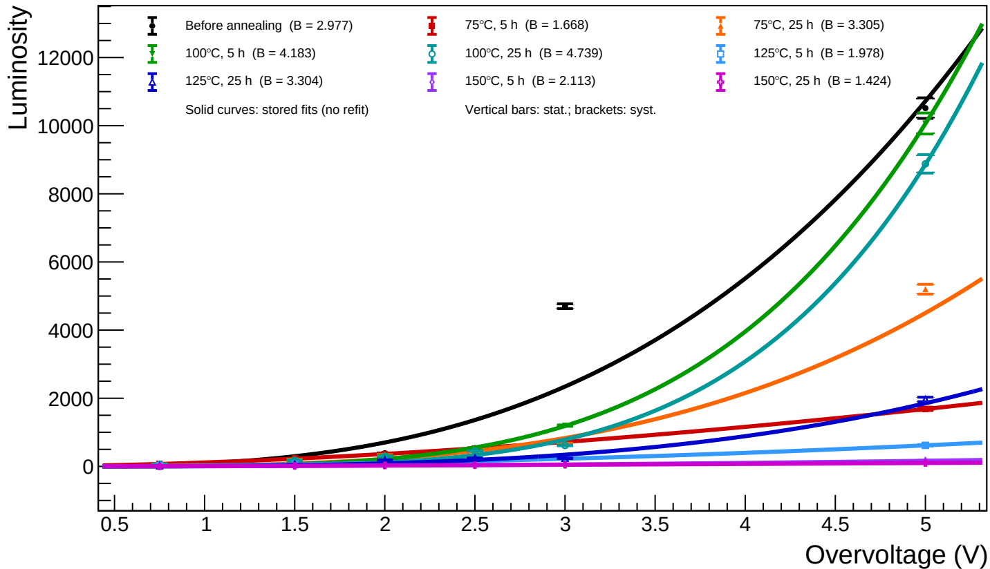
B1_T=20 - Spot 11 ( x = 347.53 , y = 554.01 ): luminosity vs overvoltage for all annealing phases
