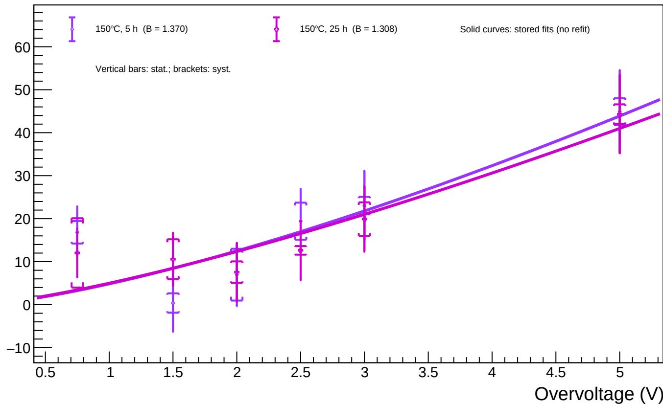
B1_T=20 - Spot 112 ( x = 1369.05 , y = 982.27 ): luminosity vs overvoltage for all annealing phases
