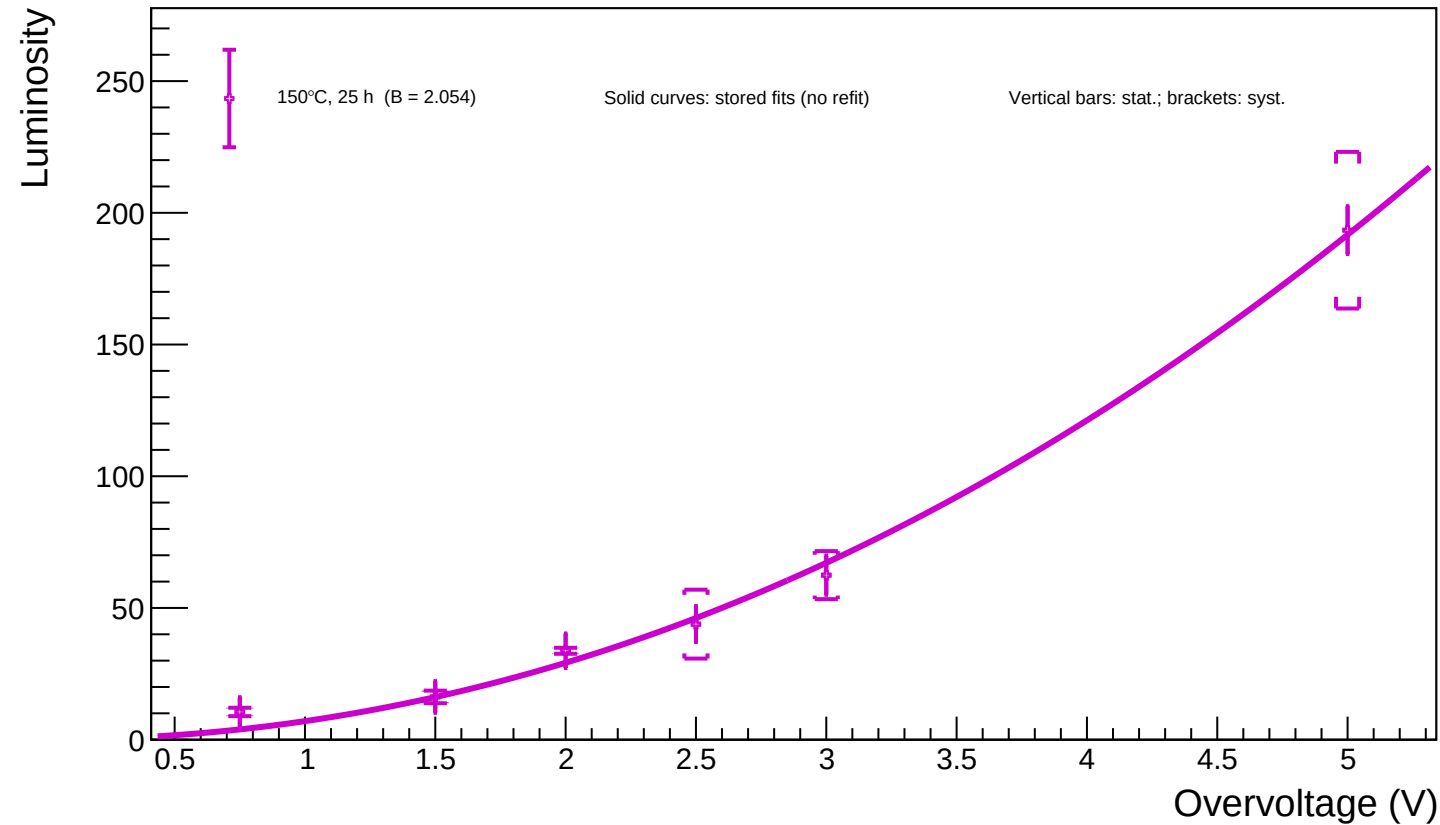
B1_T=20 - Spot 117 (x = 1032.05, y = 760.77): luminosity vs overvoltage for all annealing phases
