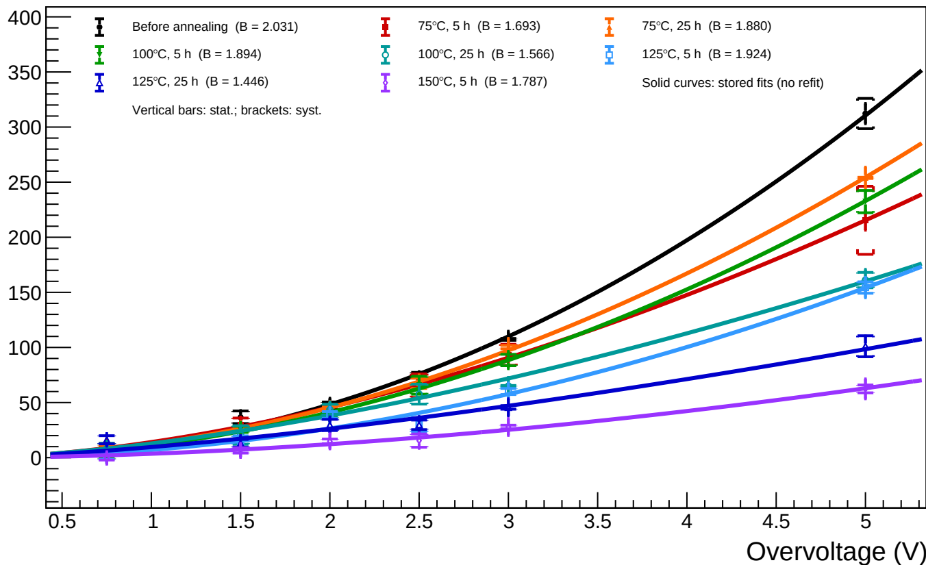
B1_T=20 - Spot 12 ( x = 347.61 , y = 391.79 ): luminosity vs overvoltage for all annealing phases
