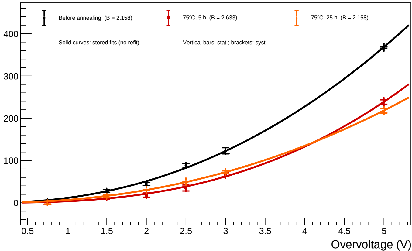
B1_T=20 - Spot 13 ( x = 352.13 , y = 710.13 ): luminosity vs overvoltage for all annealing phases
