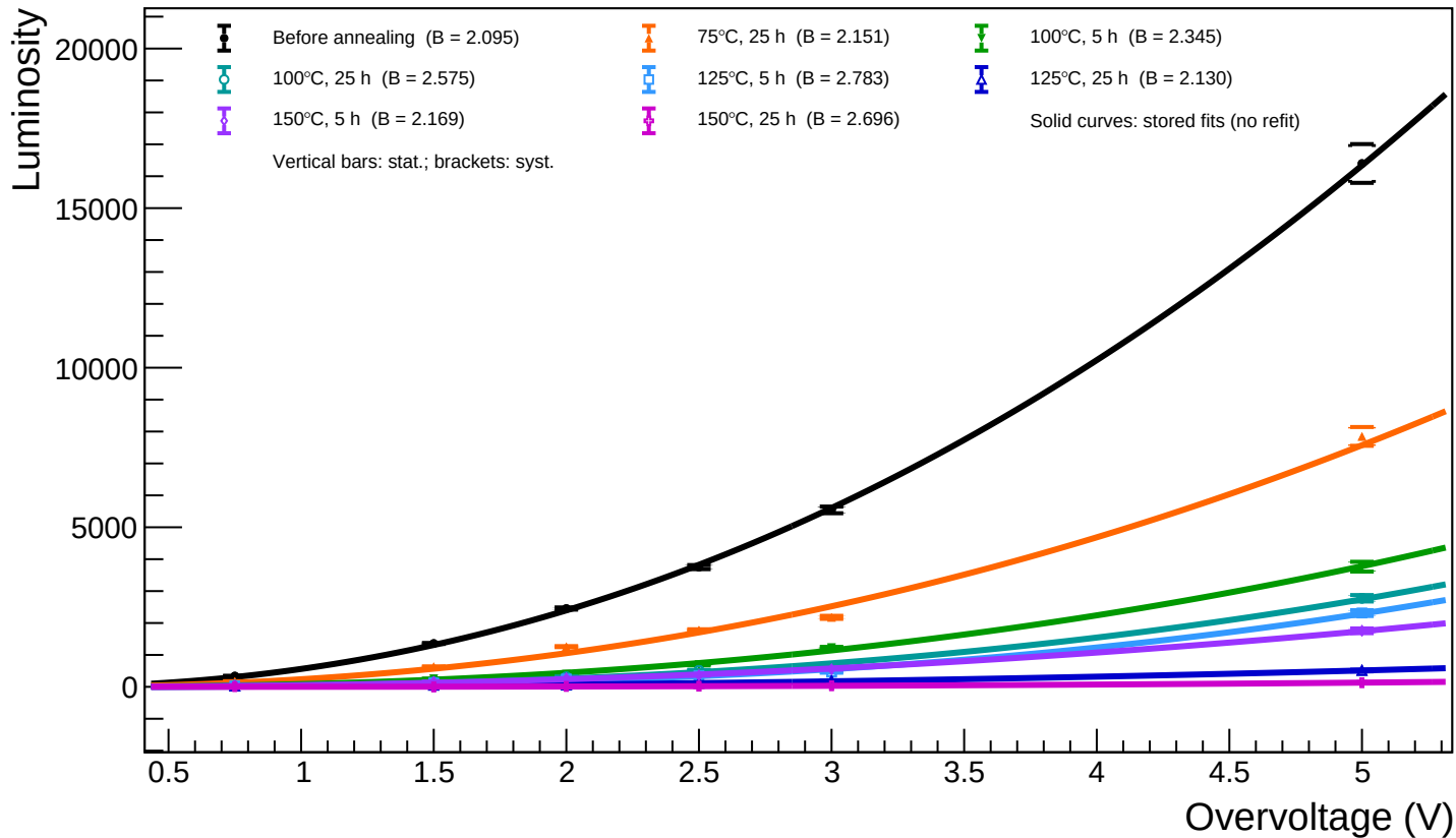
B1_T=20 - Spot 14 ( x = 390.59 , y = 830.79 ): luminosity vs overvoltage for all annealing phases
