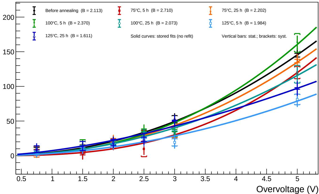
B1_T=20 - Spot 15 ( x = 405.55 , y = 529.79 ): luminosity vs overvoltage for all annealing phases
