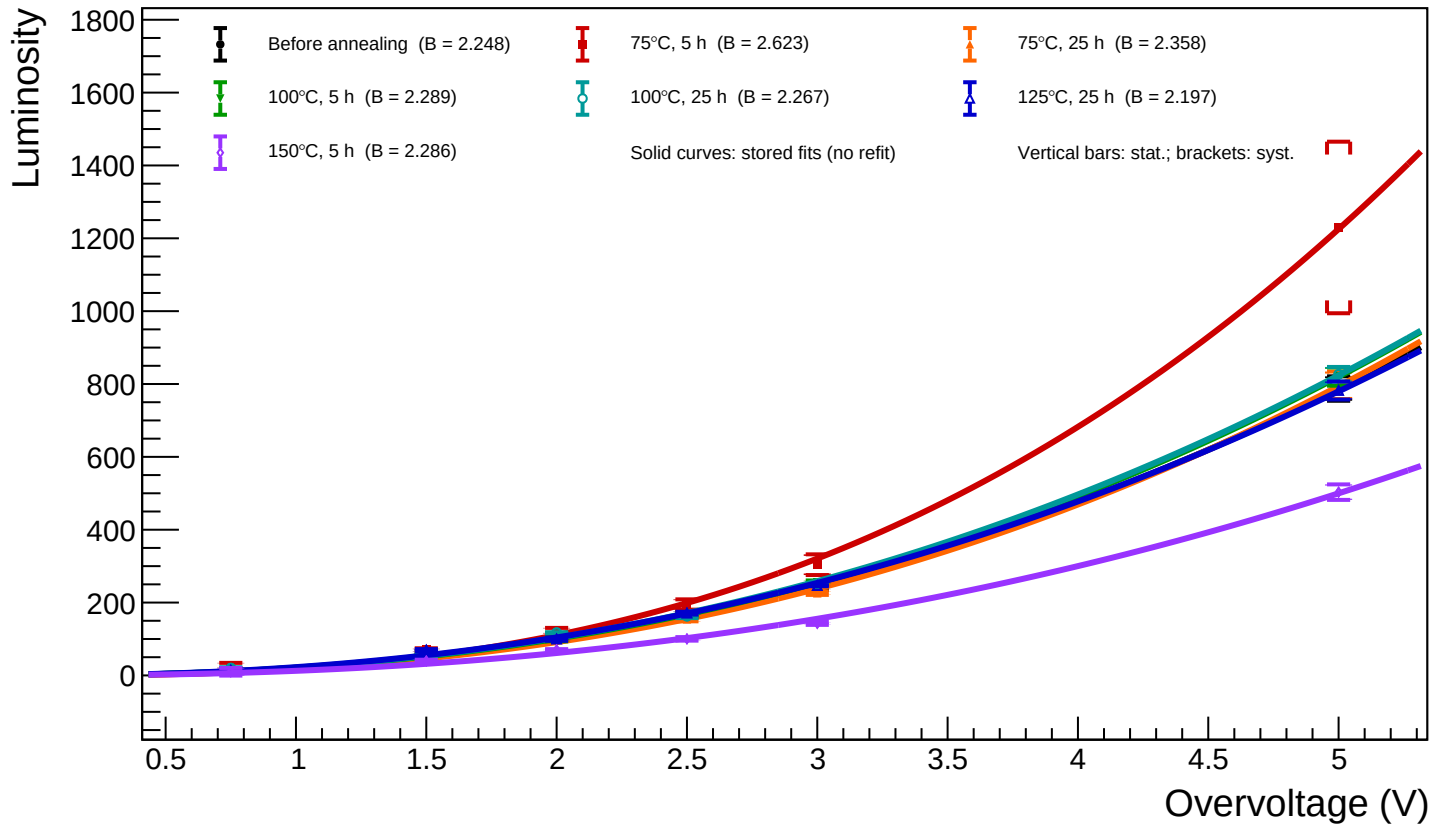
B1_T=20 - Spot 16 ( x = 458.66 , y = 828.16 ): luminosity vs overvoltage for all annealing phases
