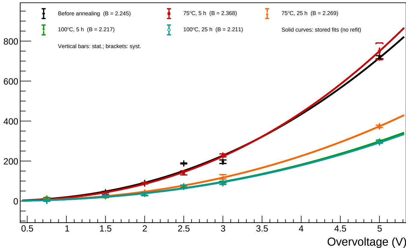
B1_T=20 - Spot 17 ( x = 460.30 , y = 888.33 ): luminosity vs overvoltage for all annealing phases
