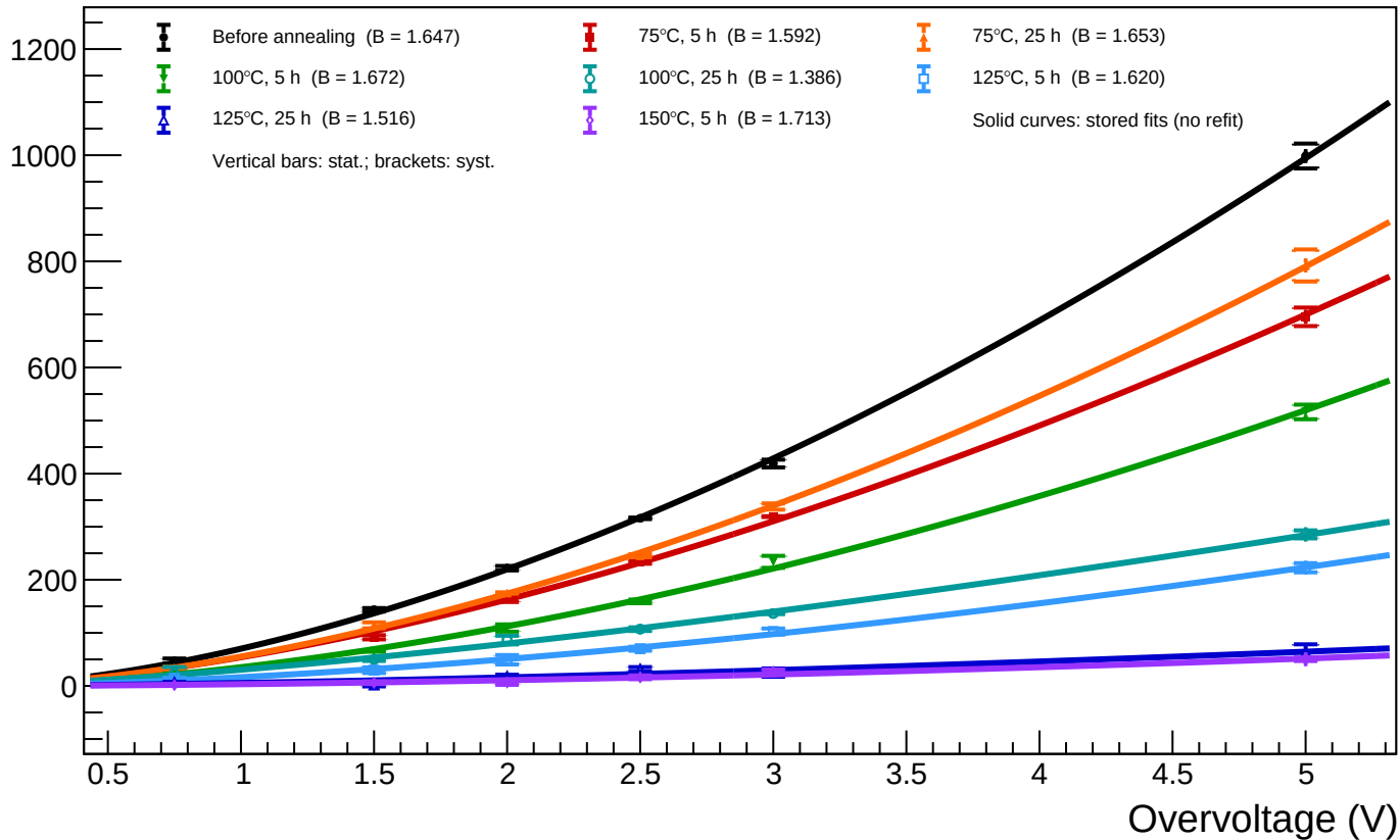
B1_T=20 - Spot 18 ( x = 472.88 , y = 339.93 ): luminosity vs overvoltage for all annealing phases
