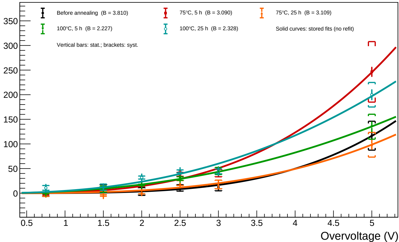
B1_T=20 - Spot 19 ( x = 490.85 , y = 668.01 ): luminosity vs overvoltage for all annealing phases
