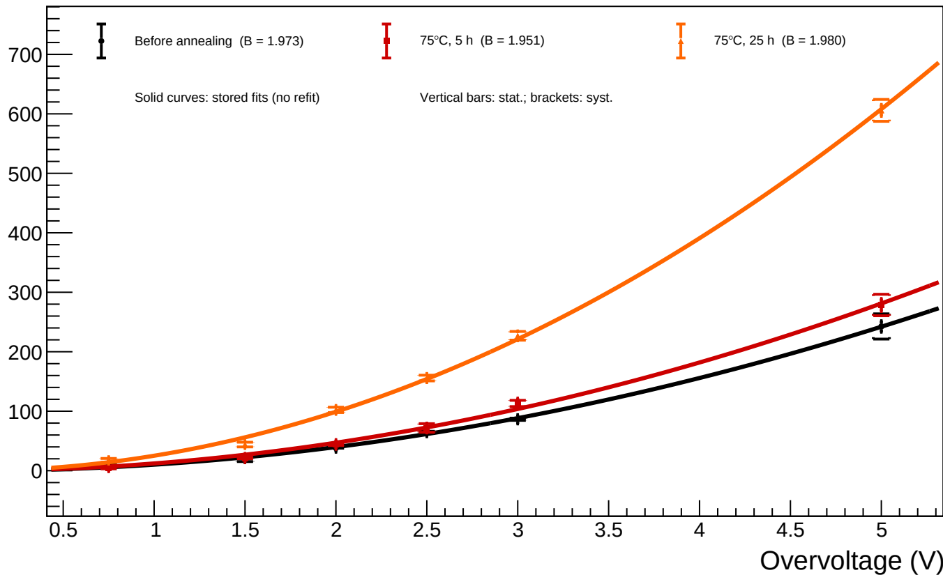
B1_T=20 - Spot 2 (x = 98.00, y = 275.50): luminosity vs overvoltage for all annealing phases
